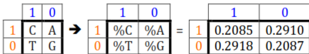
Figure 4.1.: Probabilities for A, C, G and T in Homo sapiens chromosome 1, GRCh38.p14 Primary Assembly [31], [33].
