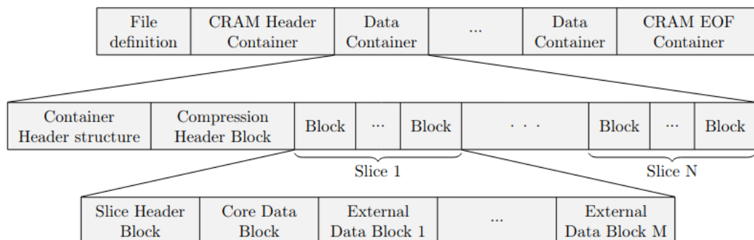
Figure 2.11.: CRAM file format structure [41].
